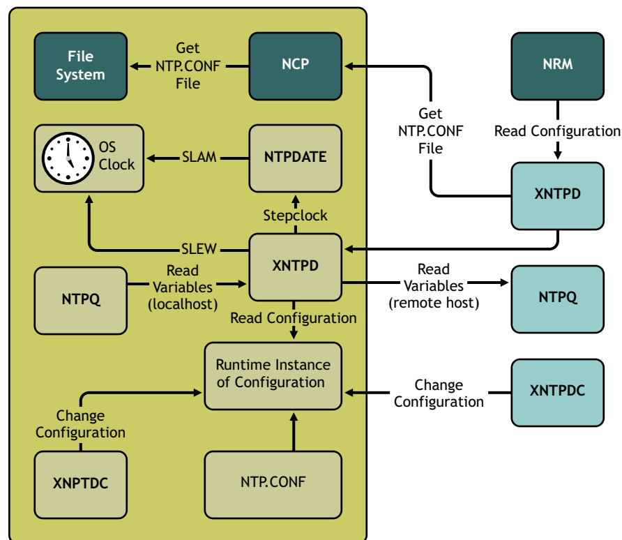
Figure 1 NTP Architecture
