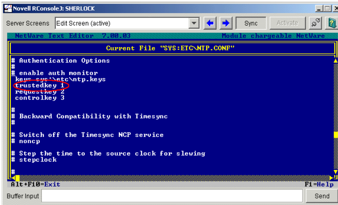
Figure 14 Ntp.conf File of ServerA
